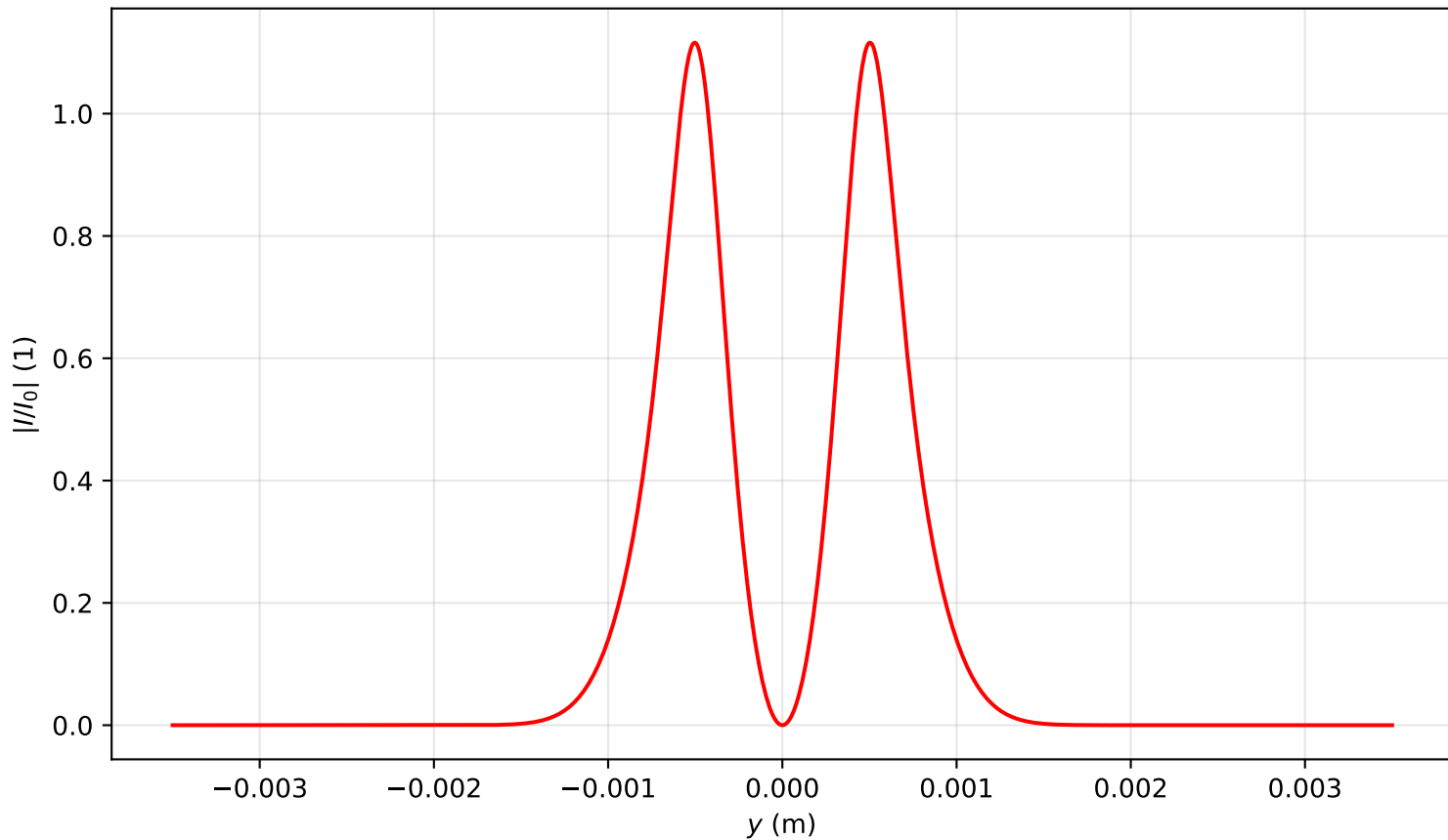
Intensity profile I(x=0, y, z=0.318)/I_0 , P_{in}=6.0P_{cr} , artificial time
